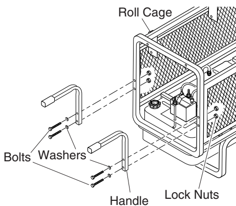
Figure 8 – Attaching Handles to Roll Cage
